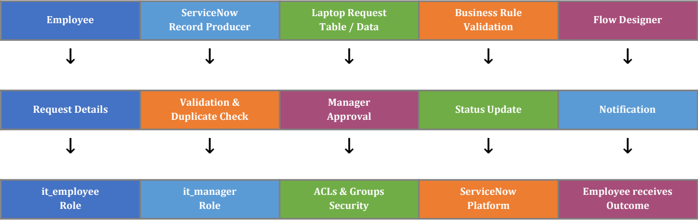
Figure 1: Architecture and data flow of the ServiceNow-Based Employee Laptop Request Application
